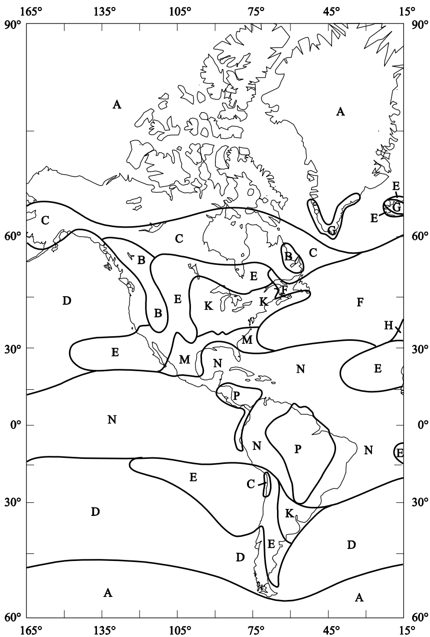
FIGURE 3 Rain-climatic zones (Region 2)
