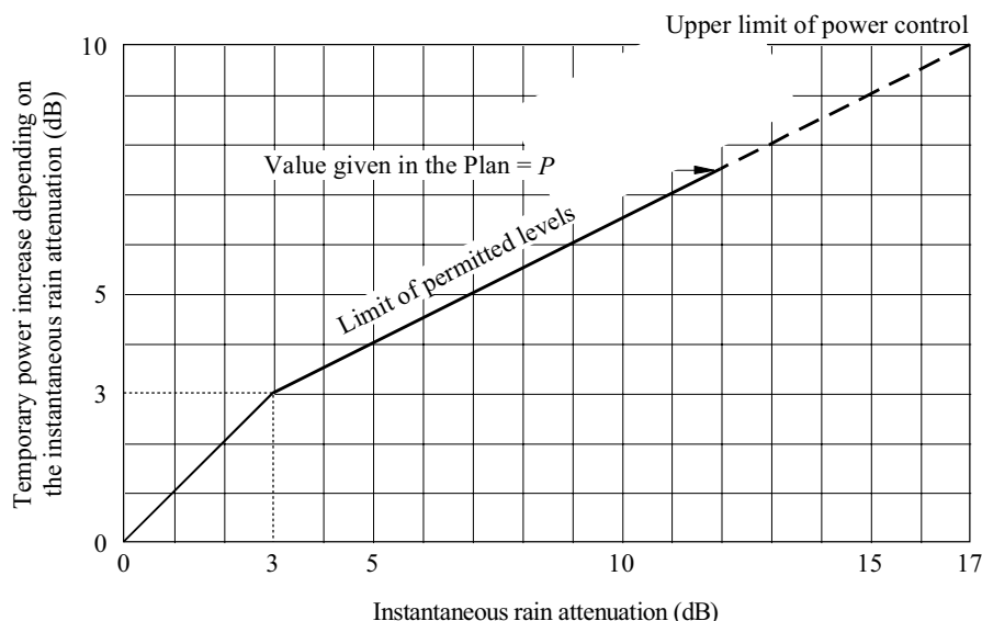
Characteristic for up-link power control
