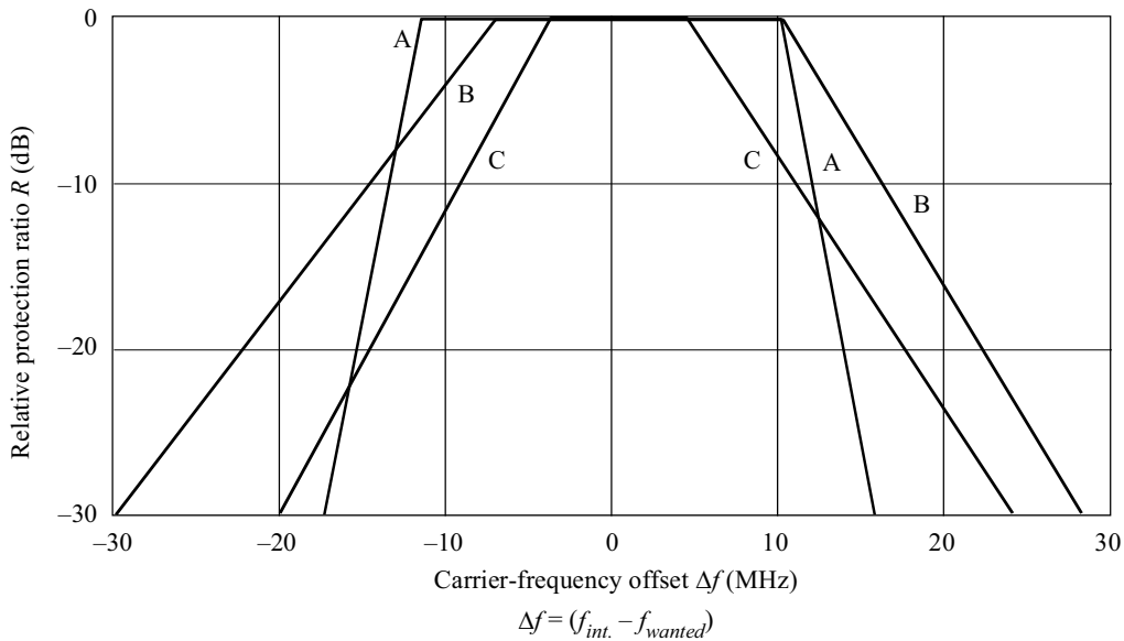
Reference case protection ratios relative to co-channel values
