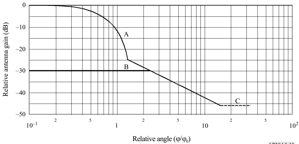
FIGURE 10 Reference patterns for co-polar and cross-polar components for satellite transmitting antennas in Region 2
