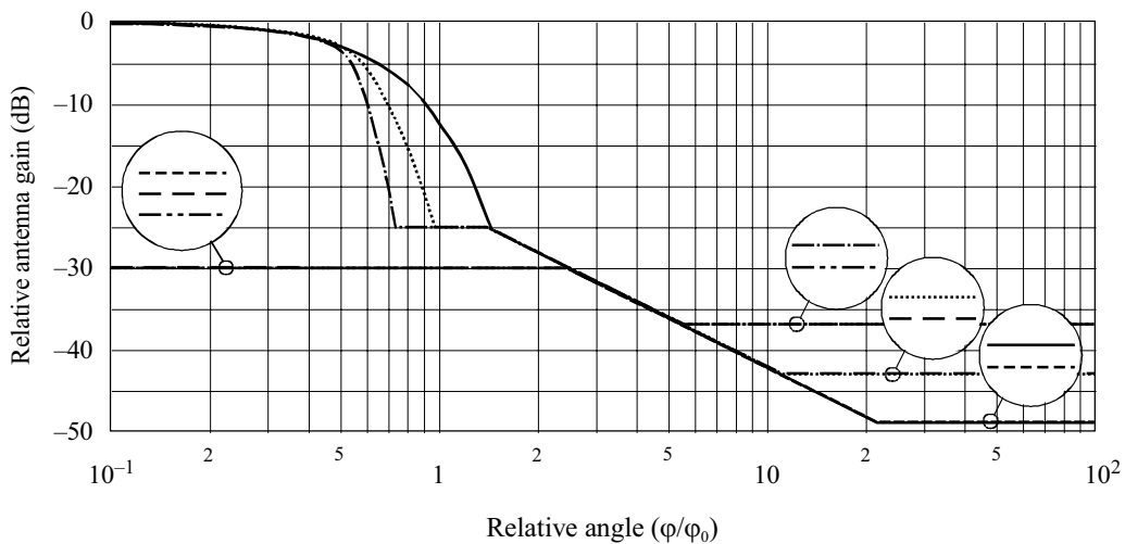
FIGURE 11B Fast roll-off antenna for Regions 1 and 3 Plan revision (beamlet beamwidth of 0.6^\circ )
