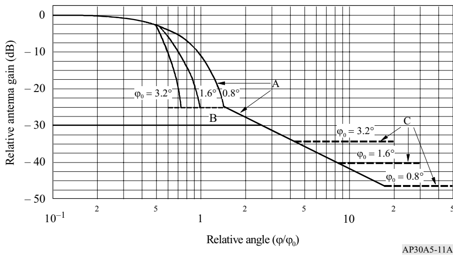
FIGURE 11A Reference patterns for co-polar and cross-polar components for satellite transmitting antennas with roll-off in the main beam for Region 2
